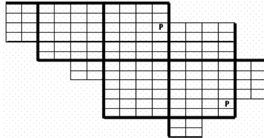
Summer Tanager 2002-2006
