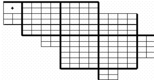
Summer Tanager 1983-1987
