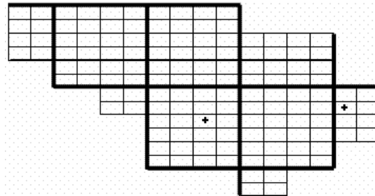
Summer Tanager 1973-1975
